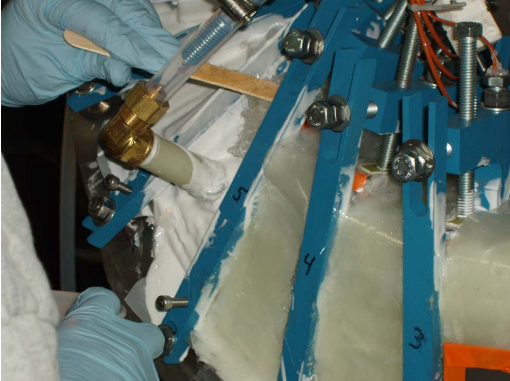
Applying Shell around Sprues
