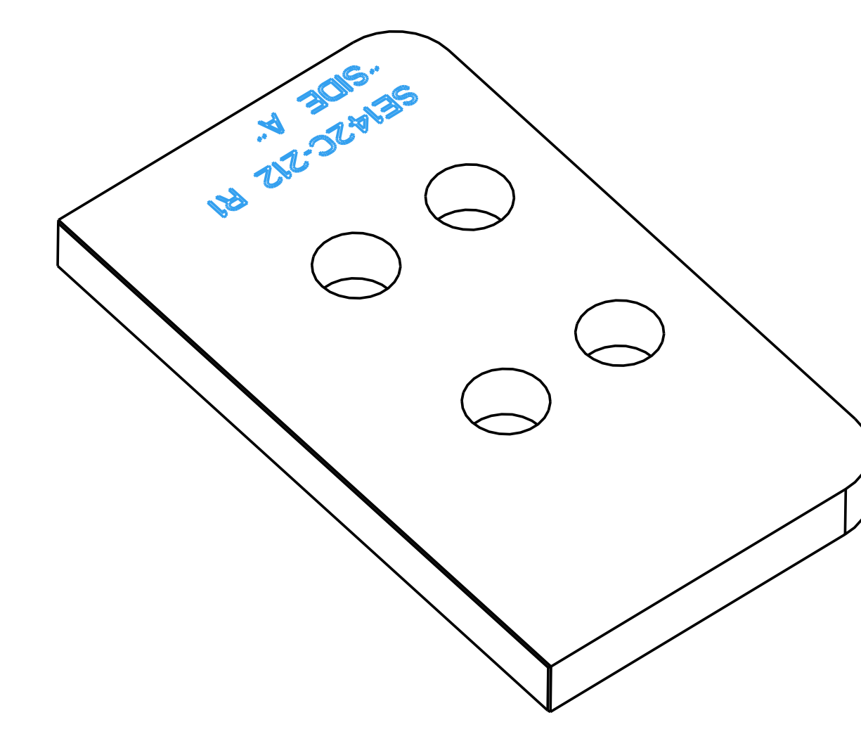
ISOMETRIC VIEW SCALE 1 : 1
