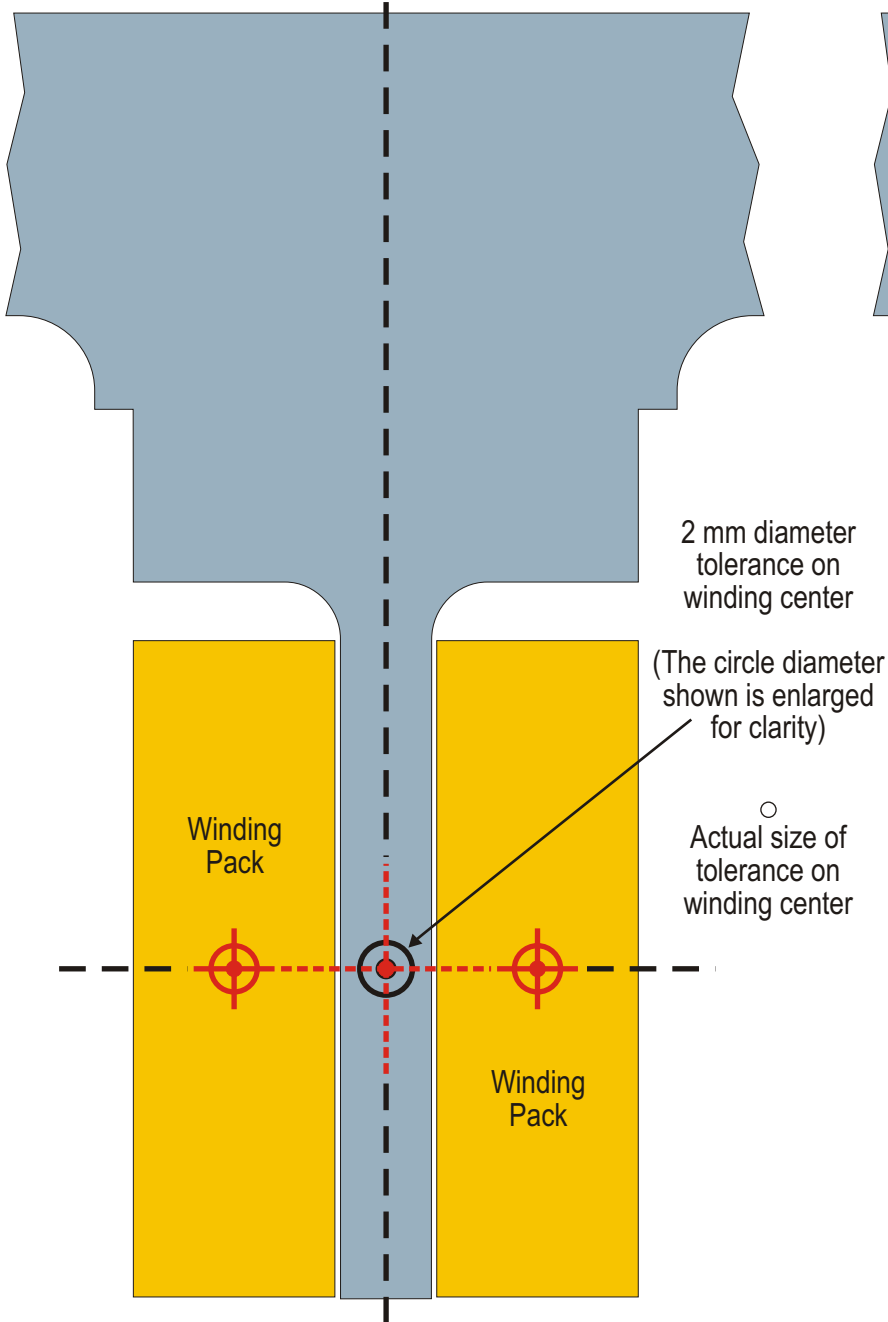
Ideal positioning and tolerancing of finished winding packs
