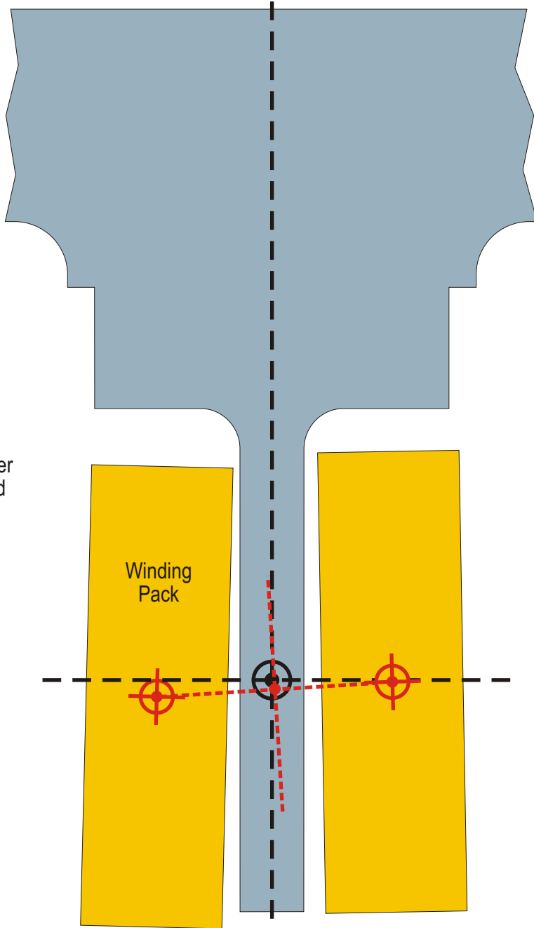
Possible misalignment of finished winding packs
