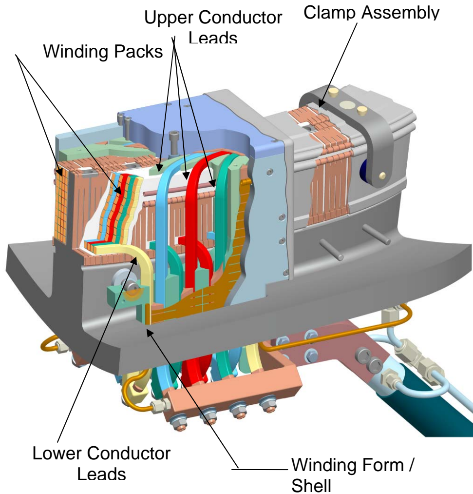
Typical Cross-section of Modular Coils at Lead Area
