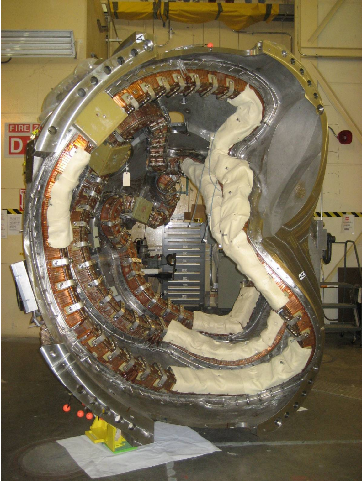
First Modular Coil 3-Pack Assembled
