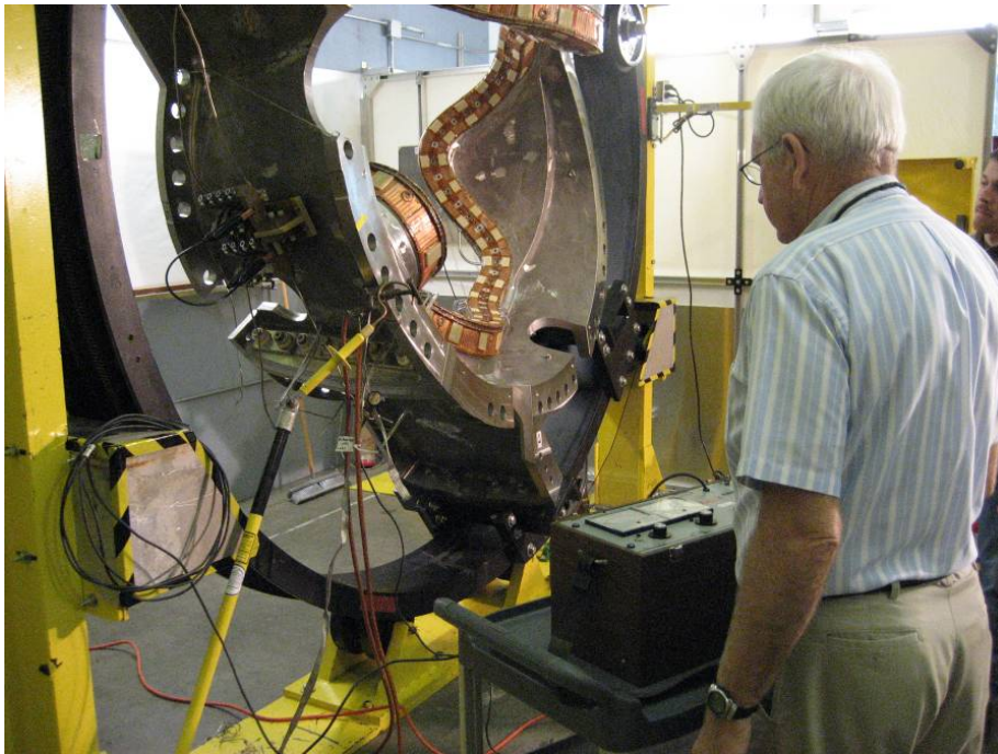
Measuring the Insulation Resistance
