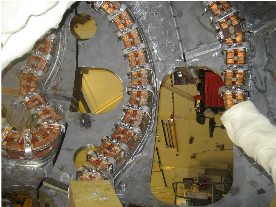
Three-Pack of Modular Coils
