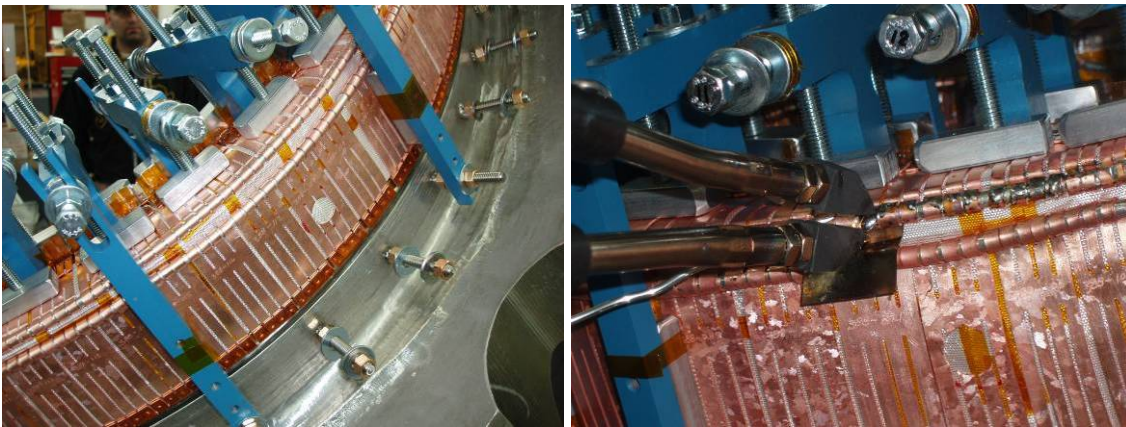
Installation of Copper Chill Plates and Tubing
