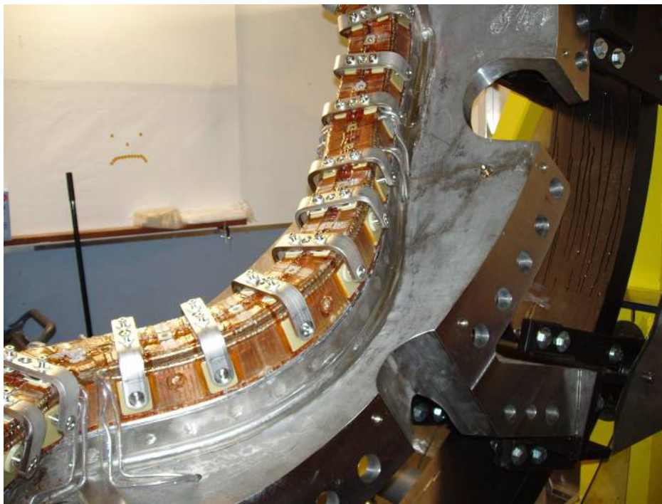
Installation of Final Clamps
