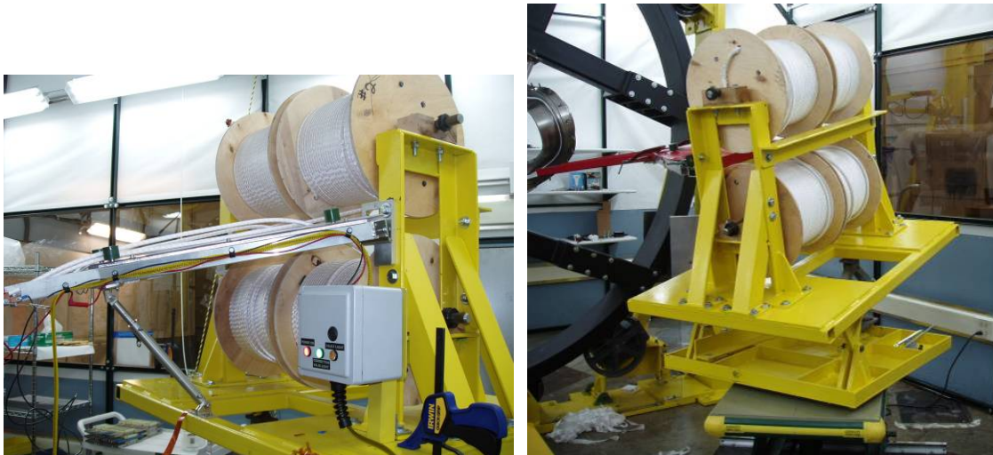
Conductor Payout Spool
