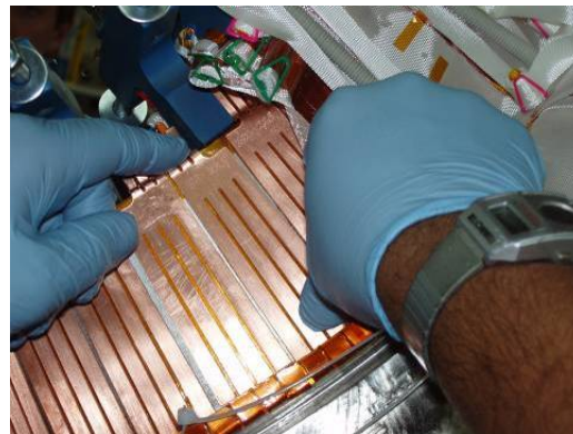
Application of 3M Adhesive to Kapton
