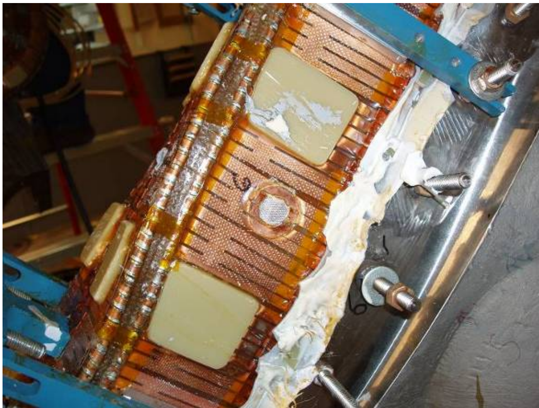
Bag Mold Removed
