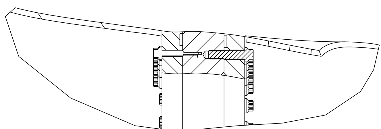
SECTION 27-27
