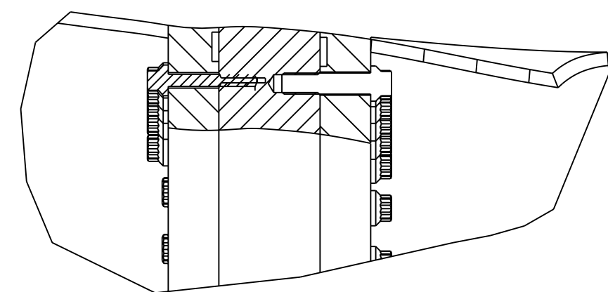
SECTION 28-28
