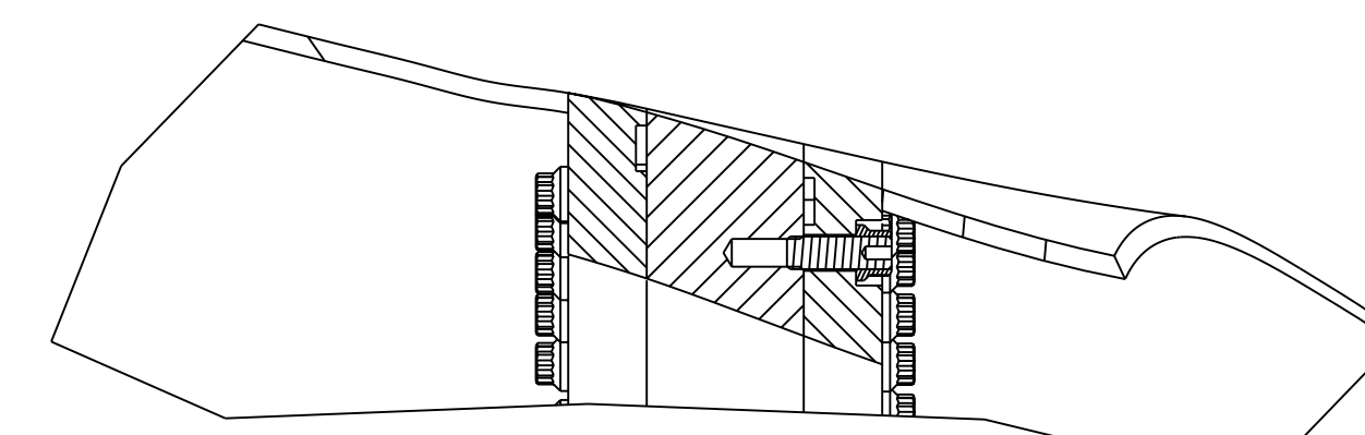
SECTION 30-30
