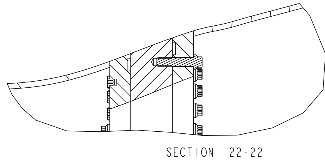
SECTION 22-22
