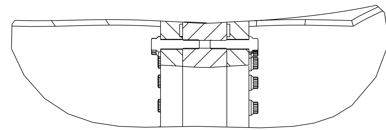
SECTION 1-1
