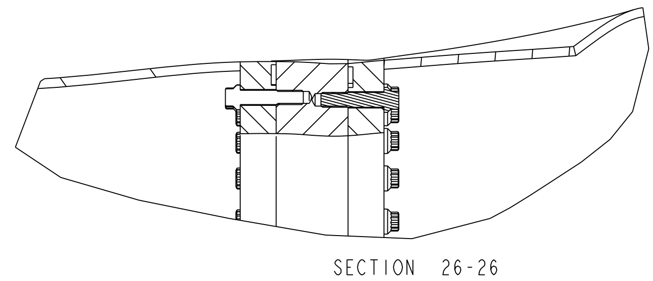
SECTION 26-26
