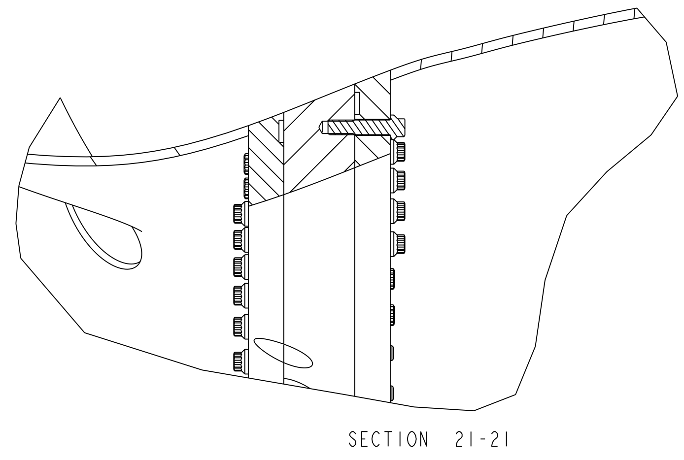
SECTION 21-21
