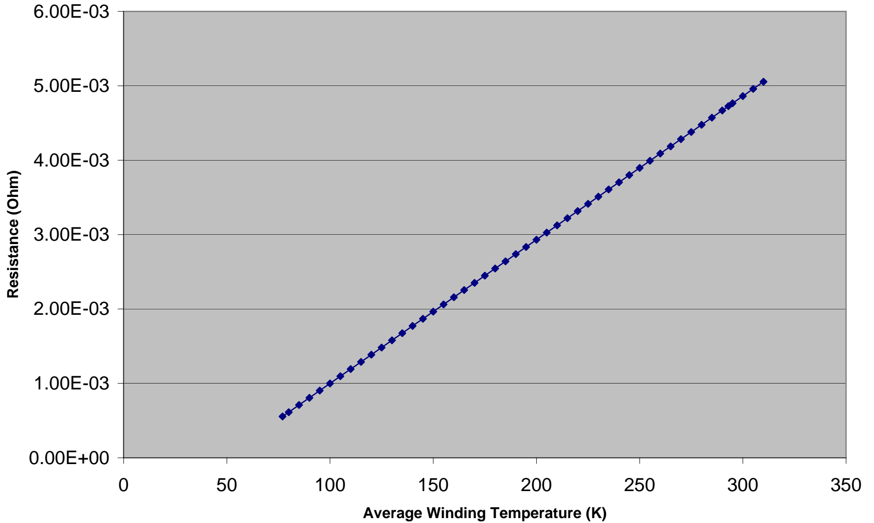
Predicted resistance vs average temperature for TRC coil
