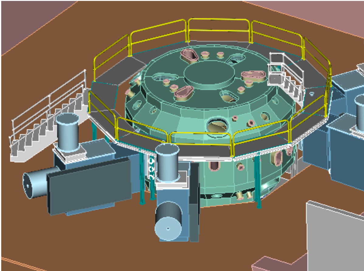
FIGURE 2-4 NCSX in Test Cell
