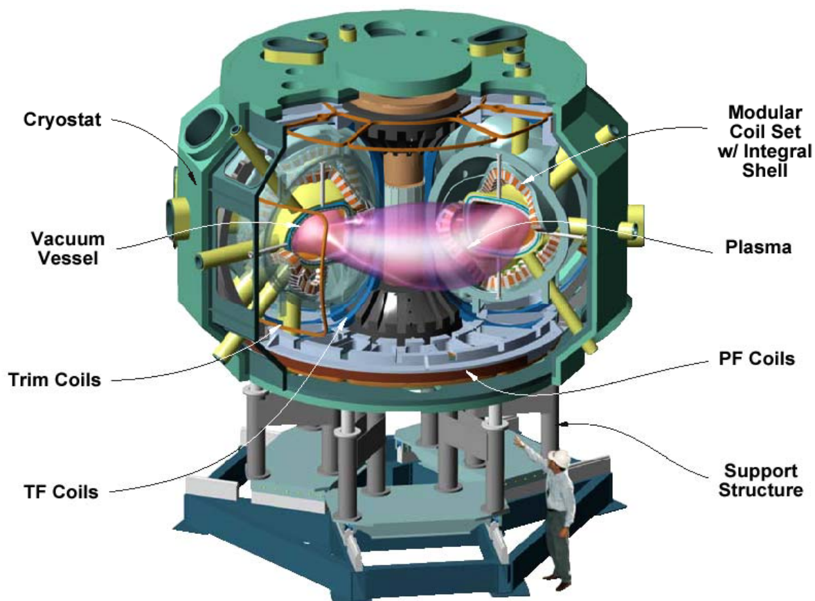
FIGURE 2-1 NCSX Device
