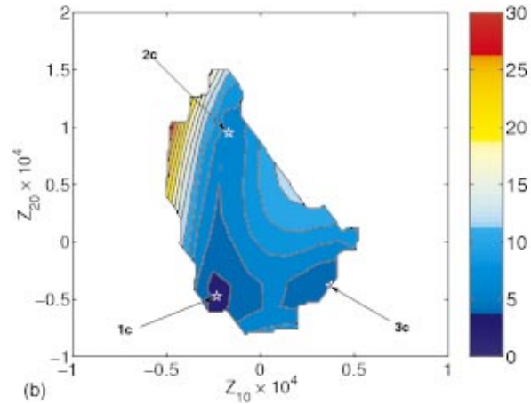
FIG. 10. (Color) Contour plots of component parts (a) \chi_\kappa(\mathbf{z}) and (b) \chi_{Bmn}(\mathbf{z}) over the (z_{10}, z_{20}) plane for the calculation of Fig. 9.
