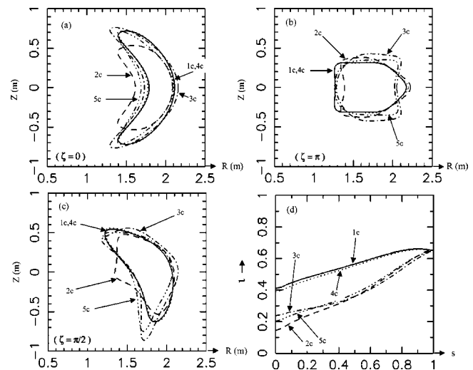
FIG. 8. Poloidal cross sections of seed configurations 1c–5c at (a) \zeta=0 , (b) \zeta=\pi , and (c) \zeta=\pi/2 . (d) Rotational transform \iota of these configurations versus s \equiv \Phi/\Phi_a .
