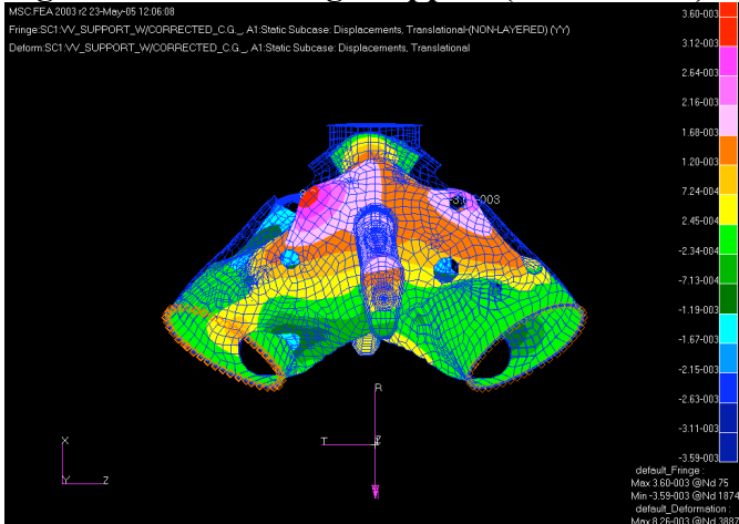
Figure 9c. Weld Flange Support (horizontal-Y)
