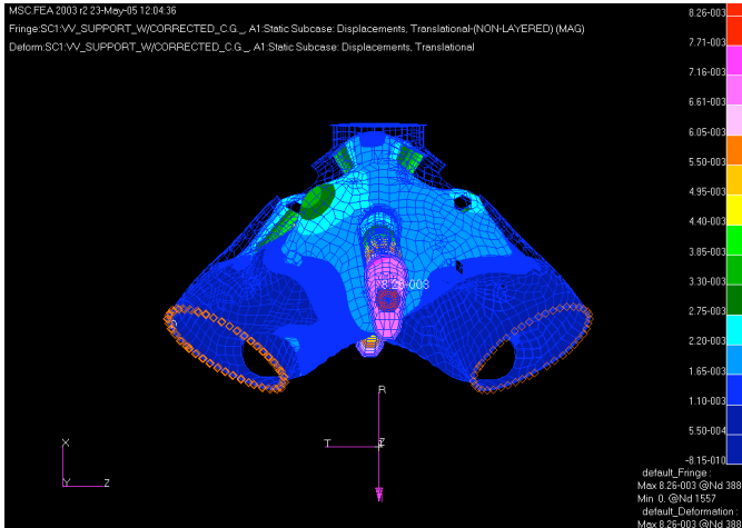
Figure 9a. Weld Flange Support (Vector-Sum)
