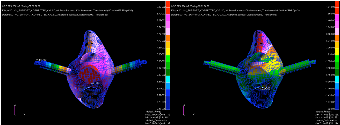
Figure 3a. Vector Sum (SRSS) displacements Figure 3b. X displacements
