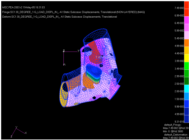
Figure 5a. Vector sum -displ.-30-degree model
