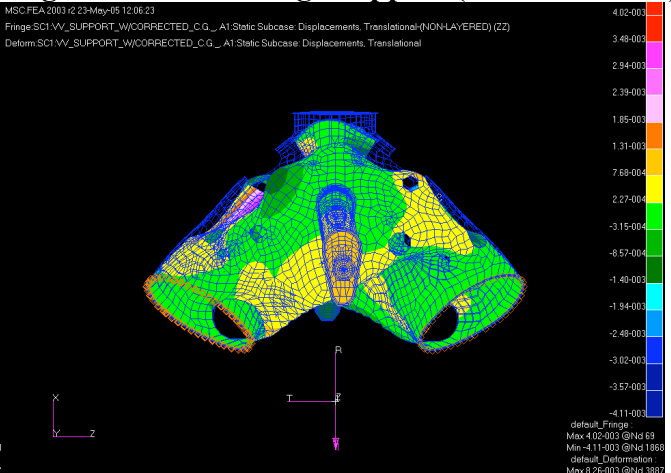
Figure 9d Weld Flange Support (horizontal-Z)
