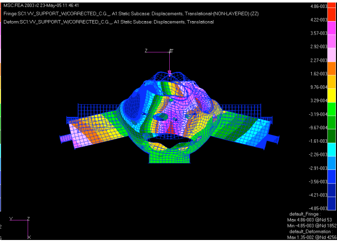
Figure 8d The Z-displacements (horizontal)
