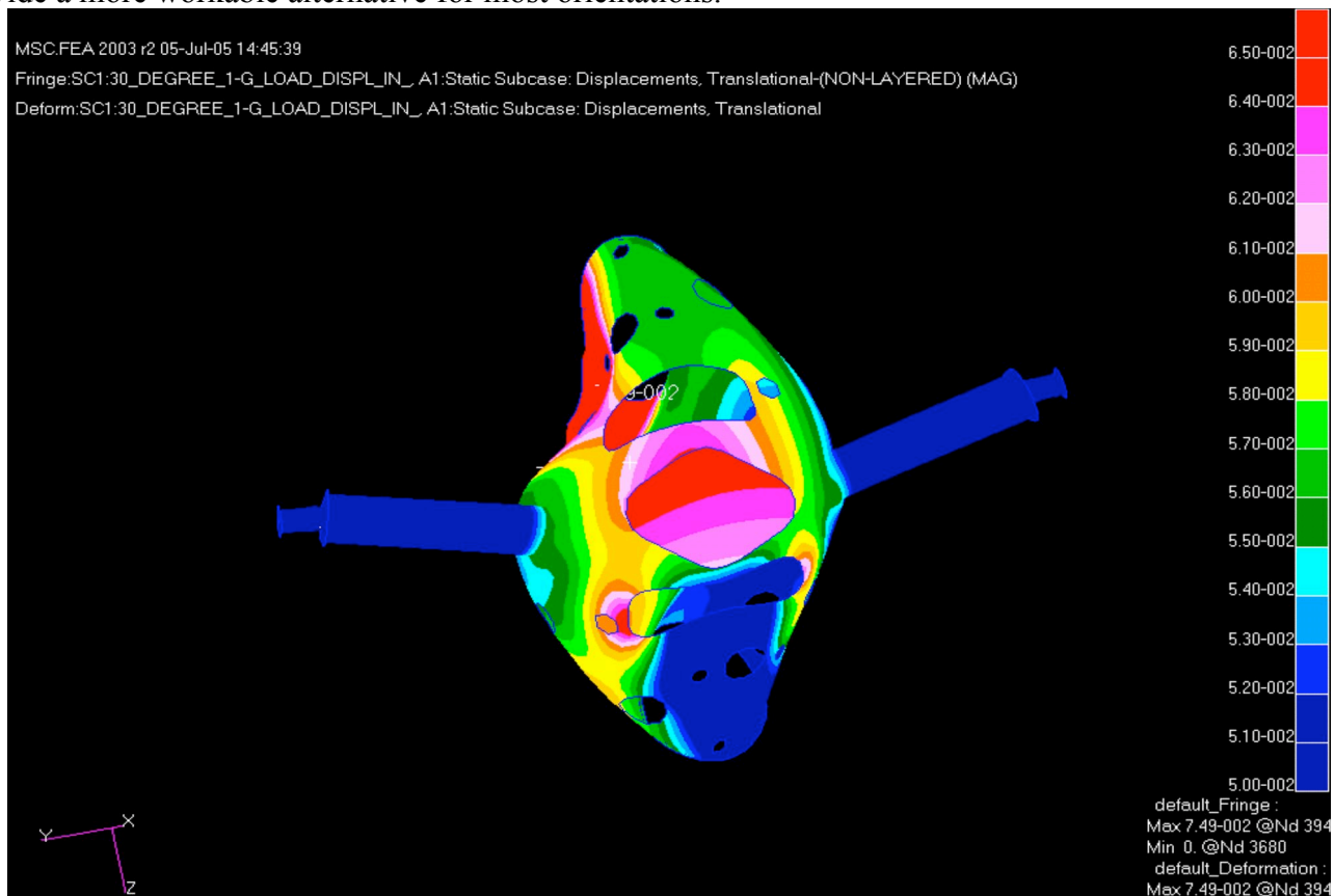
Figure 1. Contours of (SRSS) displacements at 30 degree orientation
