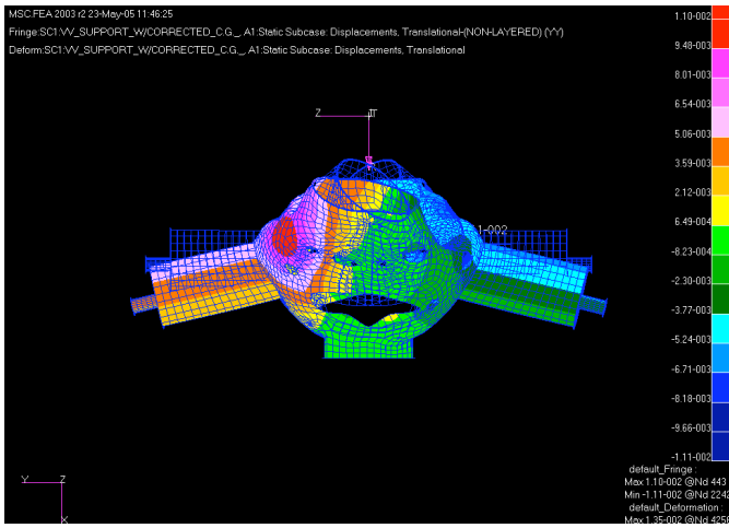
Figure 8c The Y-displacements (horizontal)
