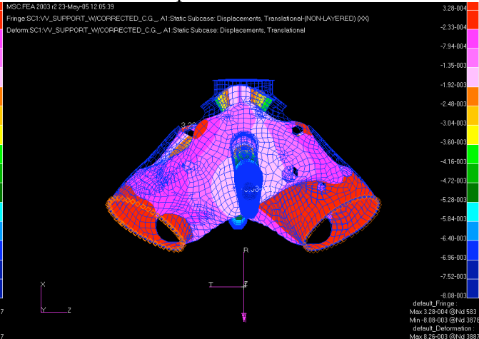
Figure 9b Weld Flange Support (Vertical- X-dir)
