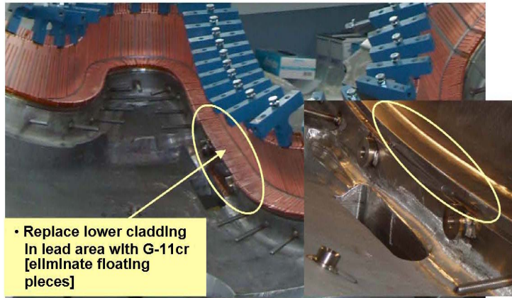
Figure 2 Lead Area Cladding- Lower
