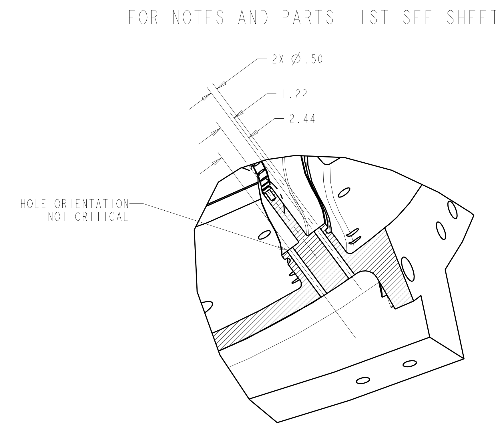
SECTION M-M
