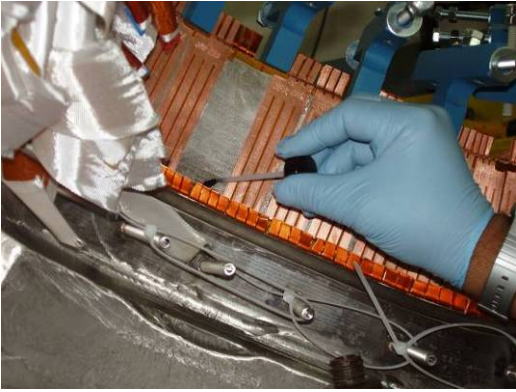
Figure 28-Applying Accelerator
