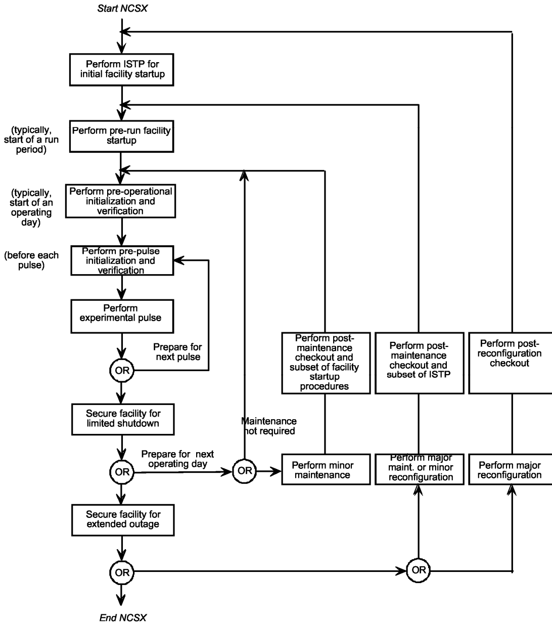
Figure 3-1 NCSX System Functional Flow Diagram
