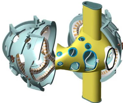
Figure 2 - Modular coils being assembled over vacuum vessel sub-assembly
